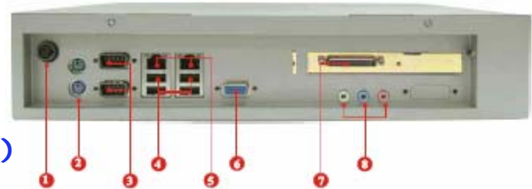
1. 12V DC-in 2. PS/2 Power Reset Button 3. Serial Ports 4. USB Ports 5. RJ-45 6. VGA Output 7. KX20 Connector to Quad DVI 8. Mic in / Line in / Line Out
