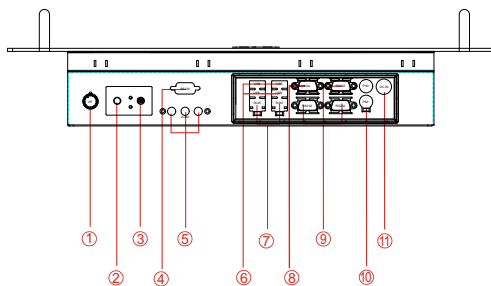
Rack Mount
