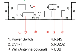
System Side IO
