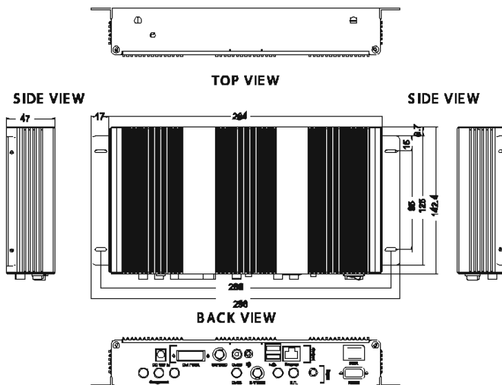
CONNECTOR VIEW
