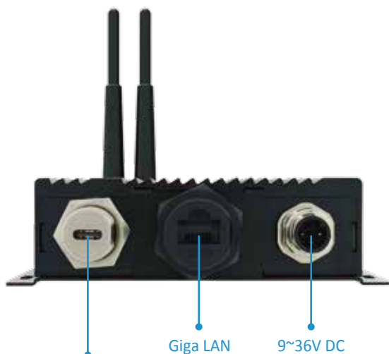
USB Type-C (Alt Mode: DP A/V Output, USB Data, Power Delivery)
